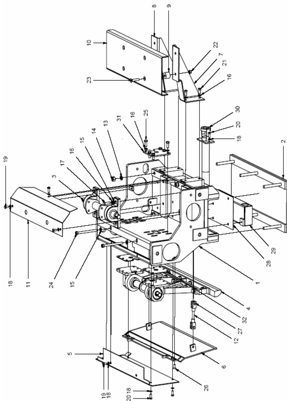
BOLTON EXTENSION 750MM - LH
