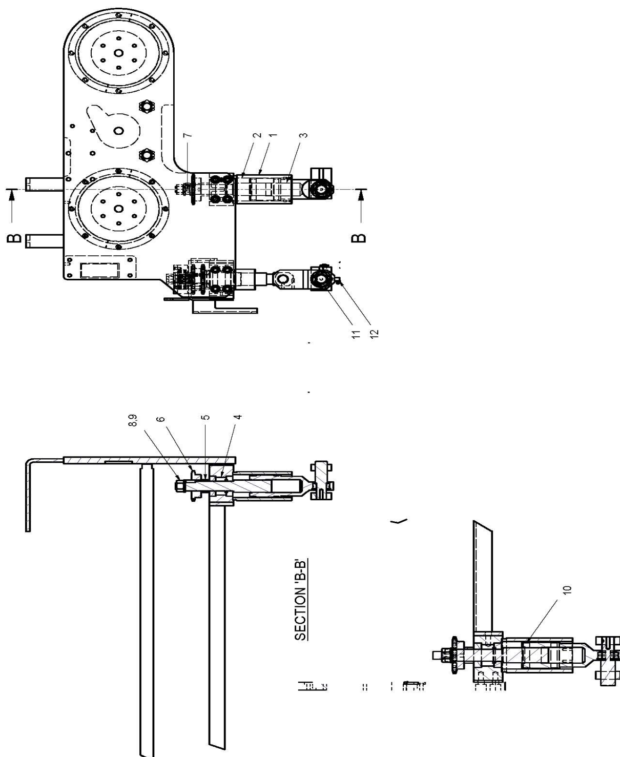
FRONT ADJUSTER SUB-ASSEMBLY (INBOARD)
