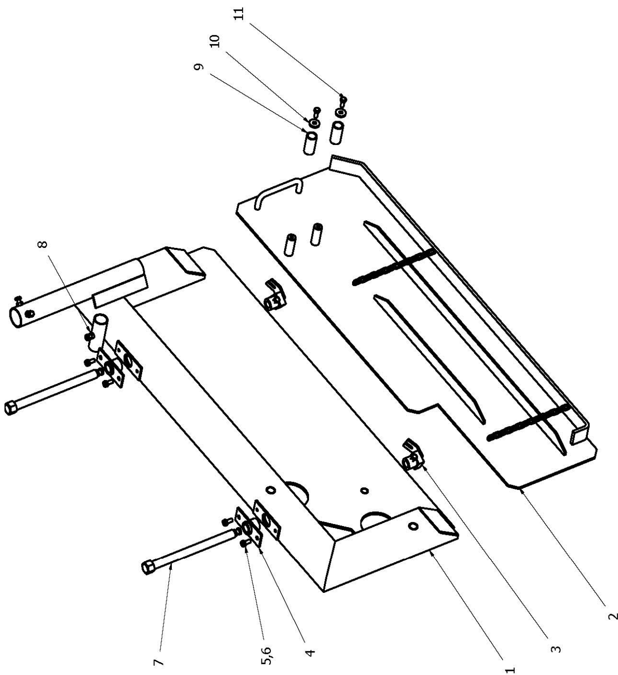
End Gate RH Complete
