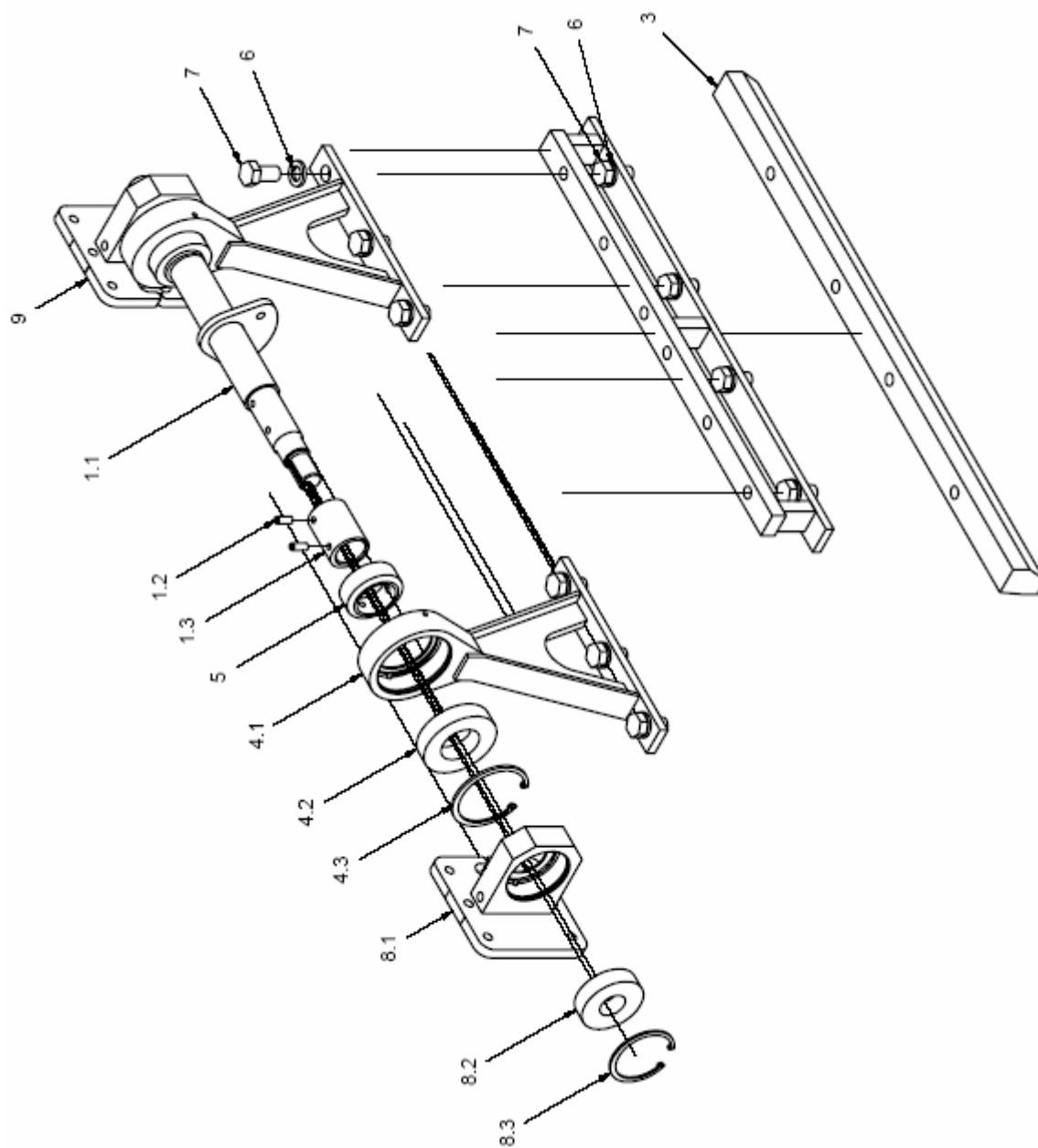
TAMPER ASSY BOLTON 750MM - LH
